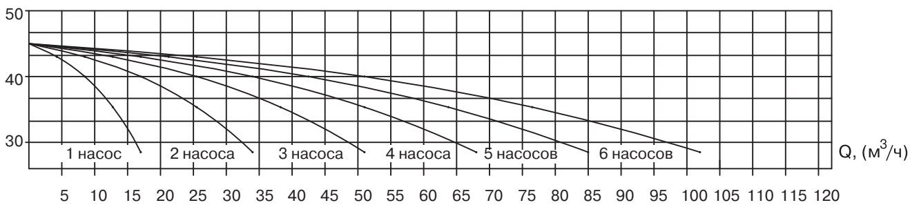
УНВ 3М 32-200/3,0
