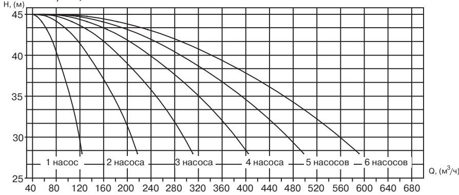
УНВ 3М 65-200/15,0
