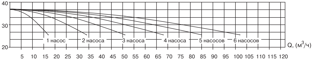
УНВ 3М 32-200/3,0
